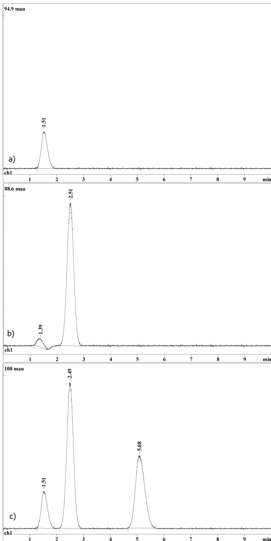
Fig. 1. Typical chromatograms of a) — “blank” solution; b) — model solution № 5; c) — test solution. Peaks with a retention time up to 2 minutes — systemic and unidentified peaks of the dosage form; with a retention time of about 2.5 minutes — sodium benzoate; a peak with a retention time of 5.08 — thioctic acid.
