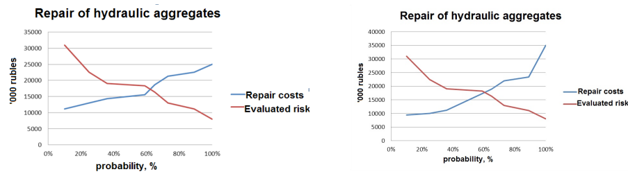
Fig. 3 Analysis of capital repair cost and evaluation of risk of hydraulic aggregate failure
