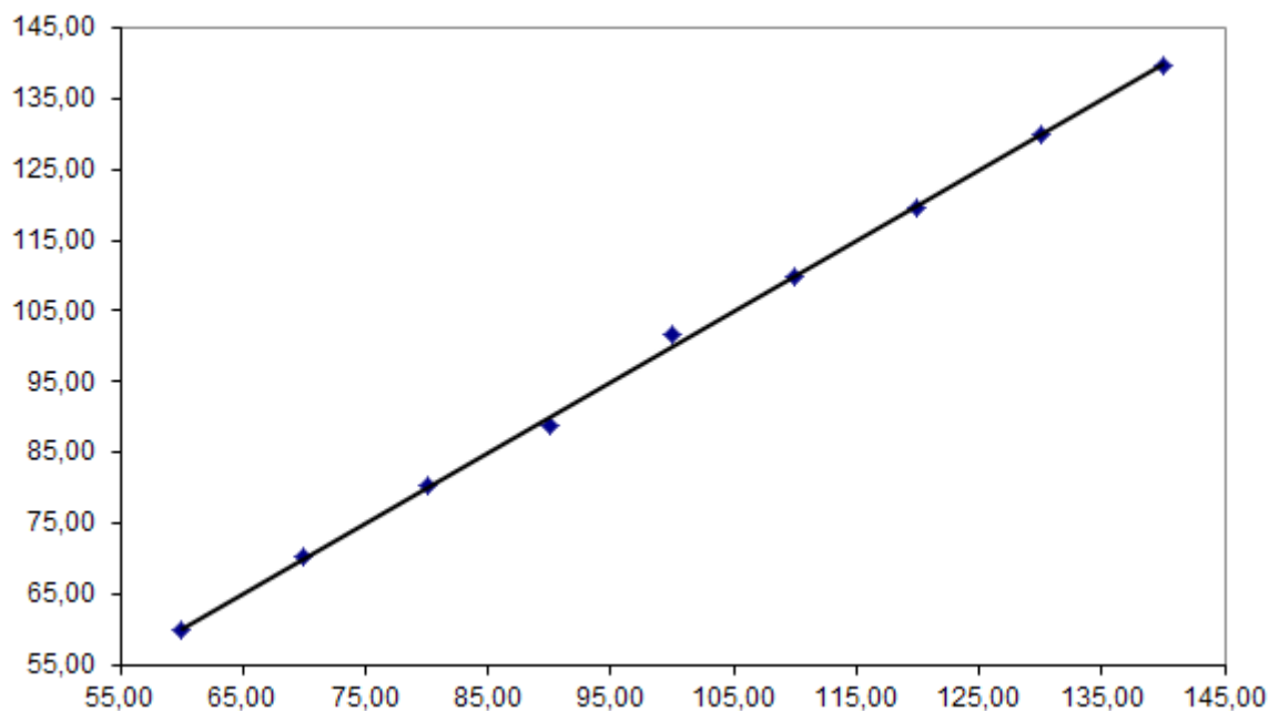
Fig. 2 The calibration line of the peak areas dependence of sodium benzoate in model solutions on its concentration in them.
